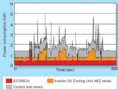
Power consumption with Hybrid System
